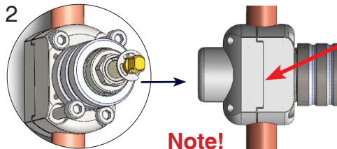
2 Clamp Housing using x 4 Bolts
